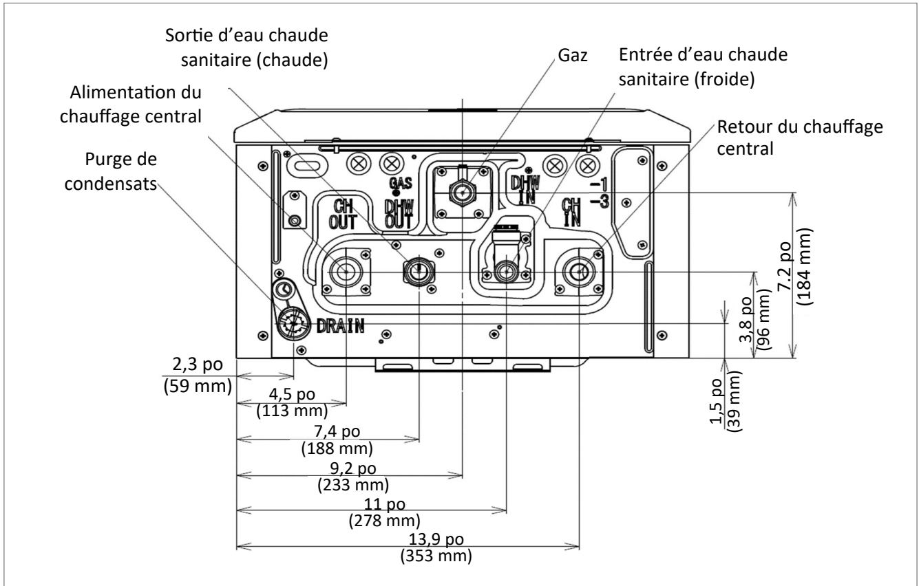
Figure 6: Raccords d'alimentation
