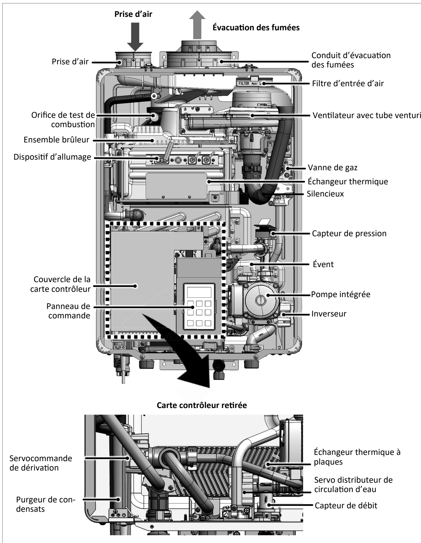
Figure 4: Composants
