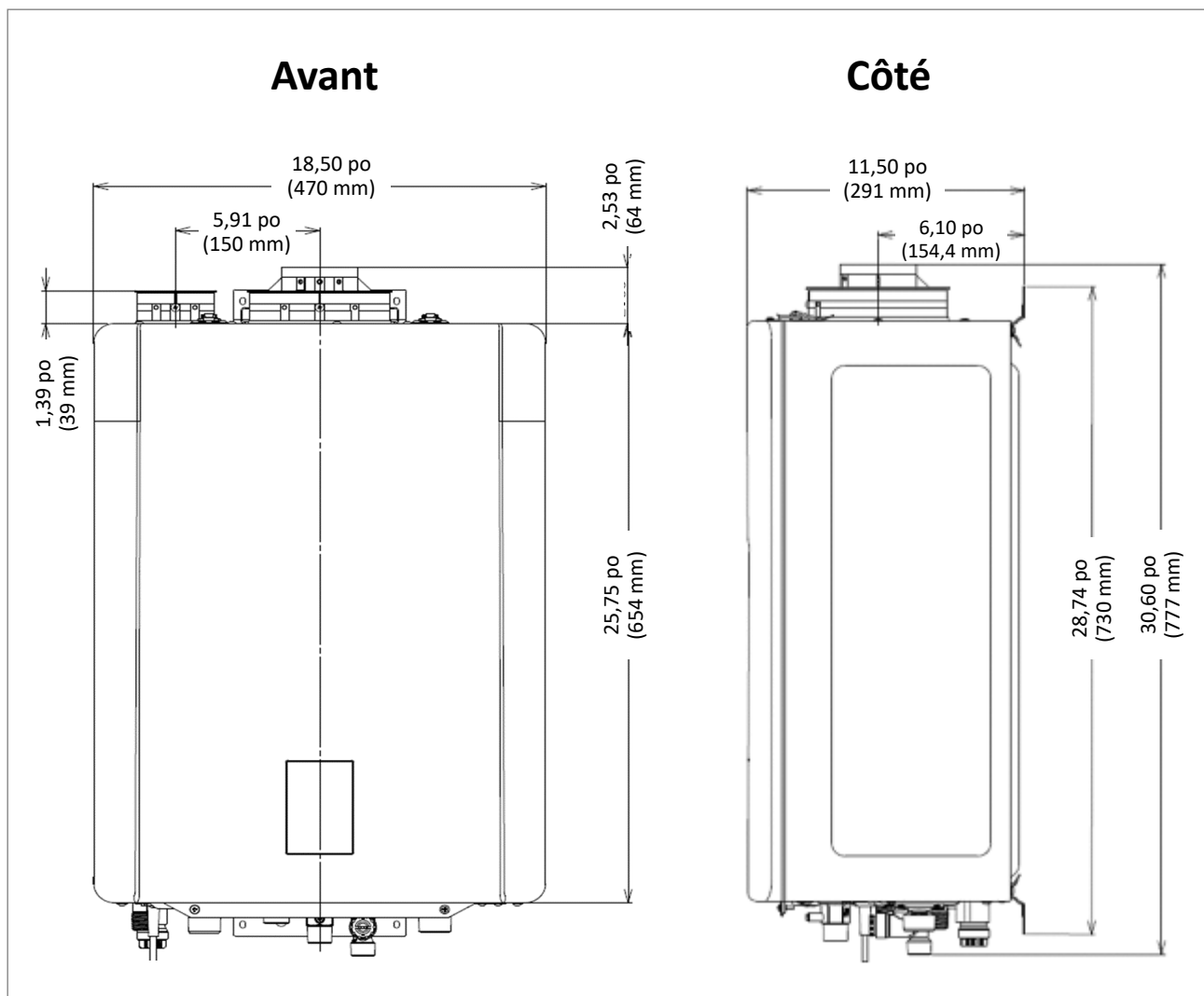
Figure 5: Dimensions
